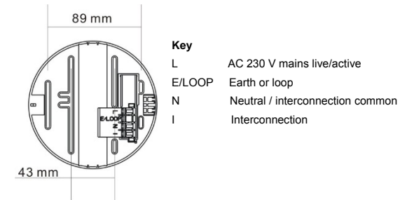
Fig. 6 – Mains wiring terminals and mounting slots
