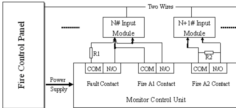
Figure 7.3 – Connection to a fire control panel
