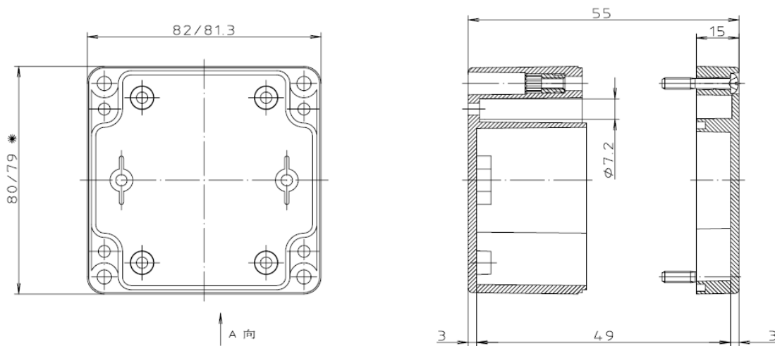
Figure 8.10 – Junction boxes
