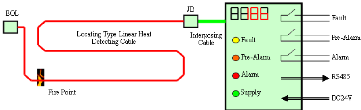
Figure 3.1 – Sensor cable and MCU configuration
