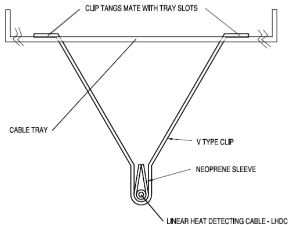
Figure 8.6 – V-type clip
