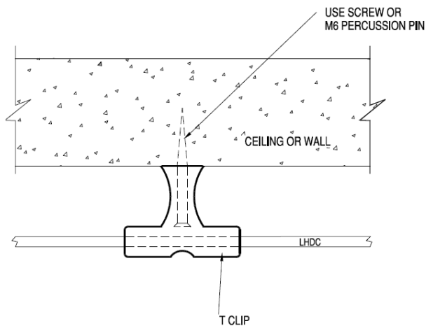
Figure 8.7 – T-type clip
