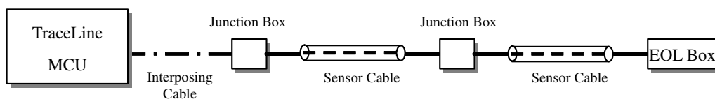
Figure 8.1 – General installation configuration
