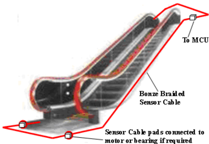
Figure 5.16 – Escalator detection
