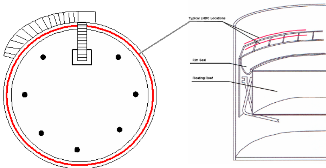
Figure 5.9 – Installation on a tank floating roof
