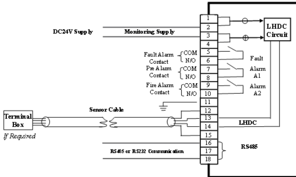
Figure 7.2 – MCU terminals
